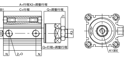
SQNJØ32~Ø100
