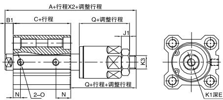
SQNJØ12~Ø25 (不附磁型)
