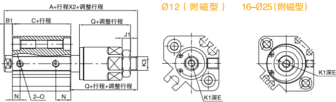
SQNJØ12~Ø25 (附磁型)
